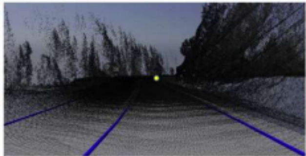
Sight Distance Analysis on Existing Highway (3-D model built from LIDAR point cloud)
